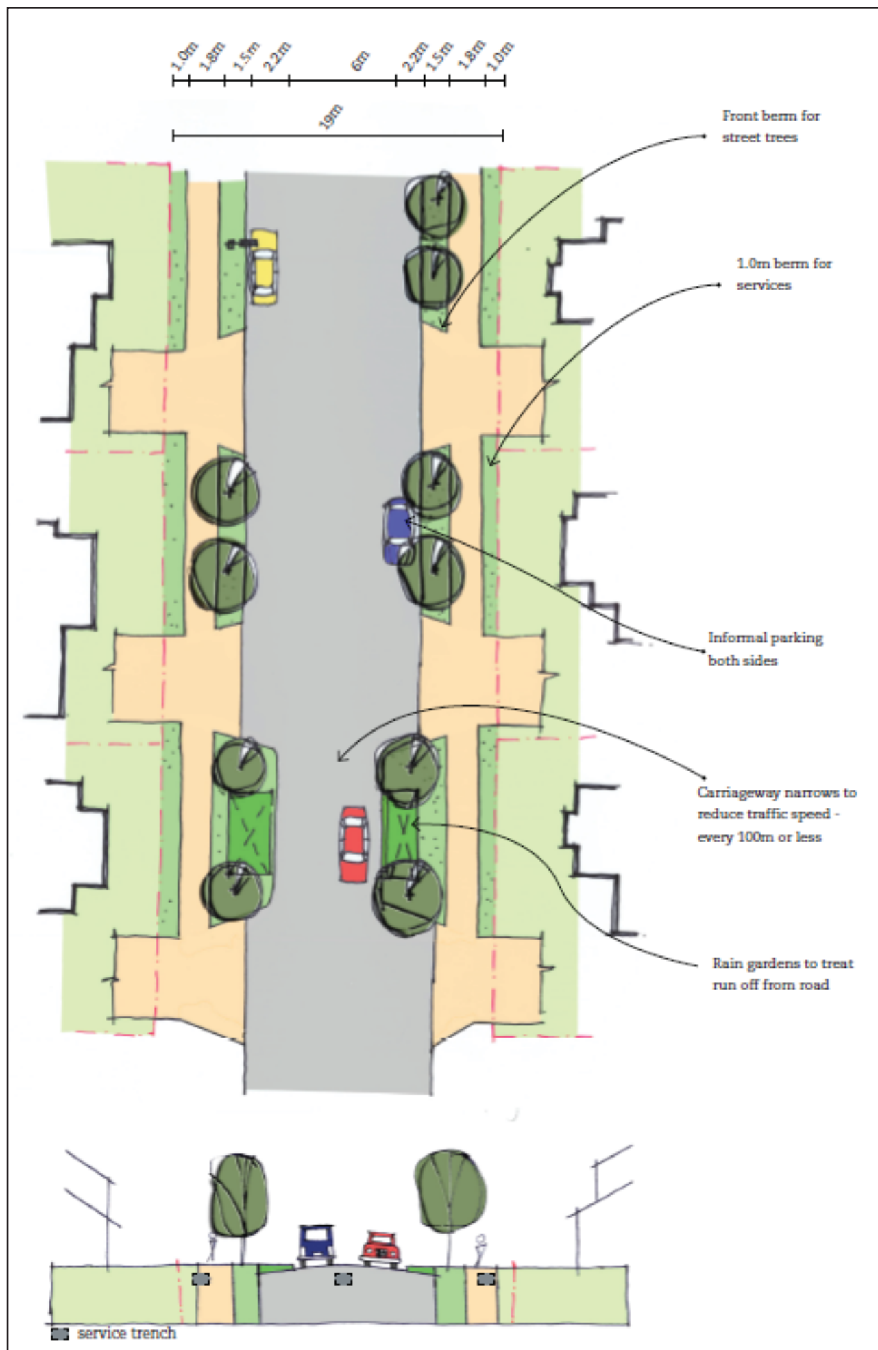
Figure 6 - Road Typology C - Key Local Road
